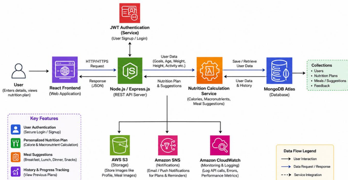
Figure 1: Solution Architecture of the Nutrition Assistant System
